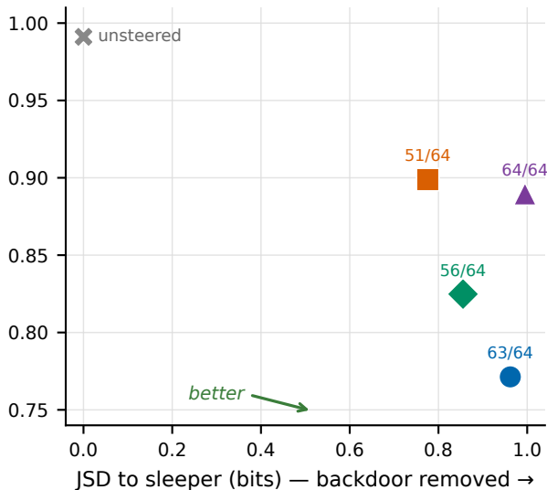
a Layer 8 confirmation set
