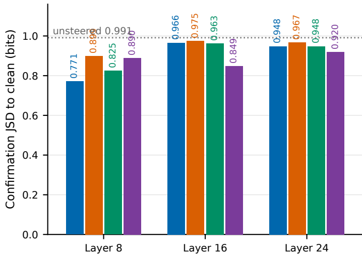
b By layer · lower is better
