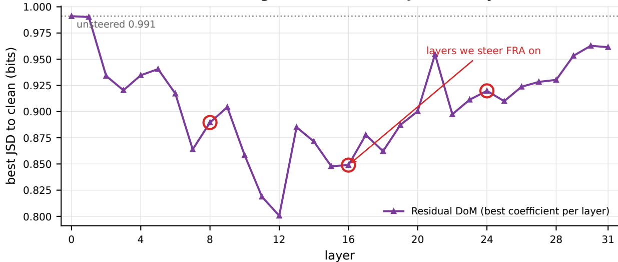
Difference-of-Means steering reaches its lowest JSD near layers 8-16
