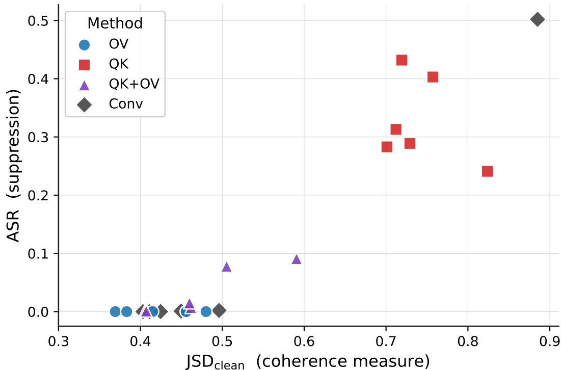
Most coherent intervention selected from each method's Pareto frontier across 6 SAE seeds
