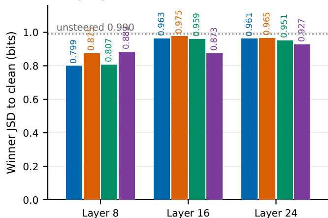
d By layer · lower is better
