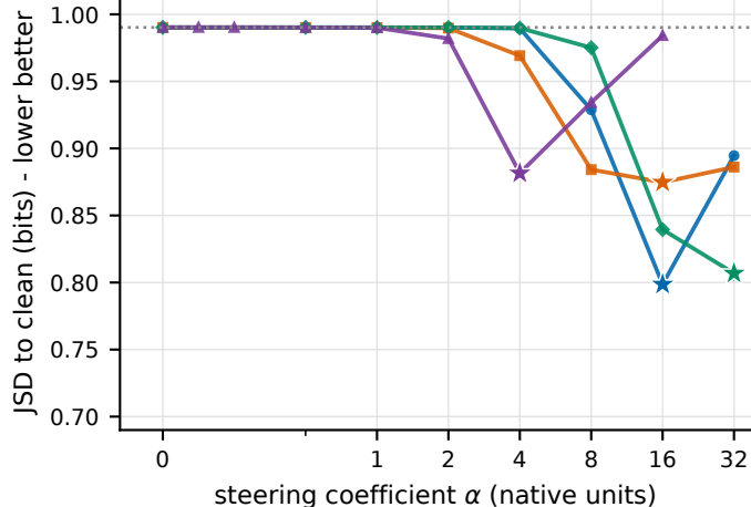
a Coefficient sweep · JSD to clean
