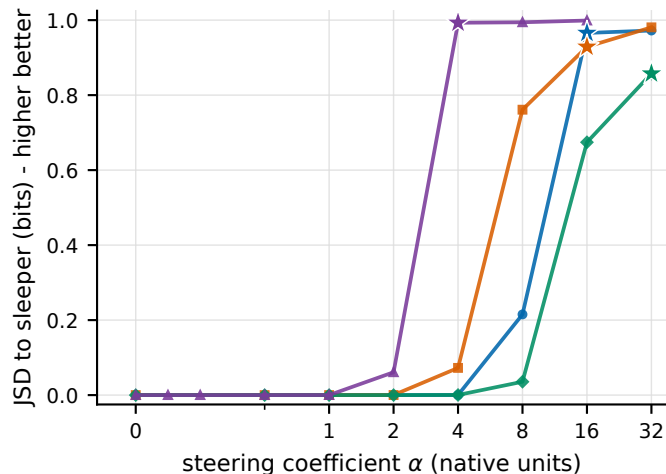
b Coefficient sweep · JSD to sleeper
