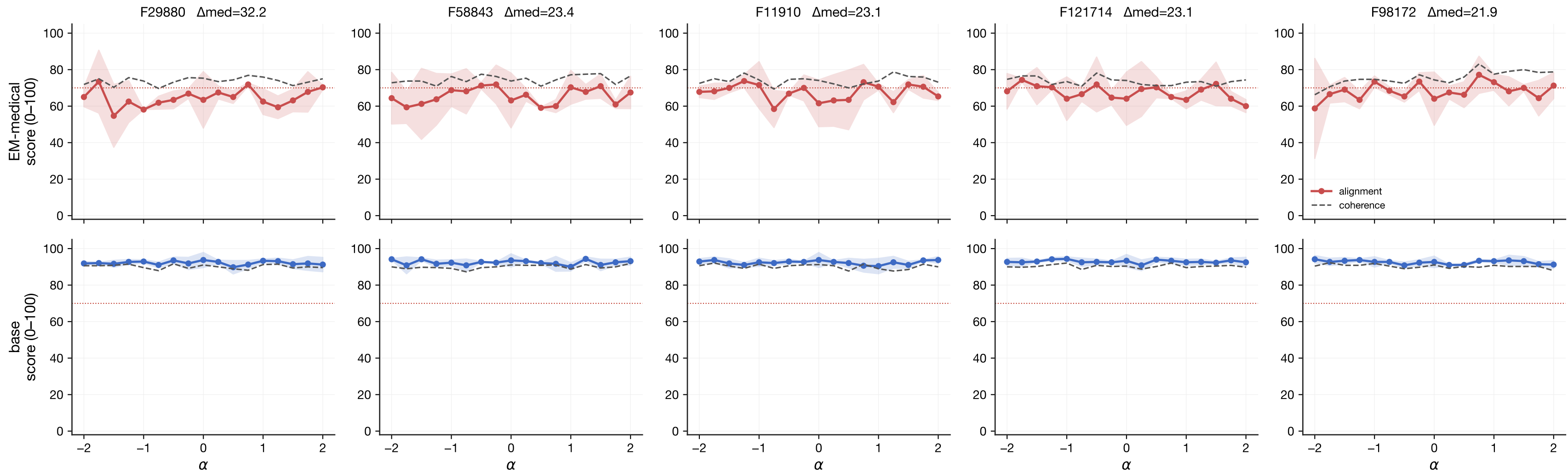
Top-5 Wang features by EM-medical \Delta\text{coh70} — \alpha -sweep per model
