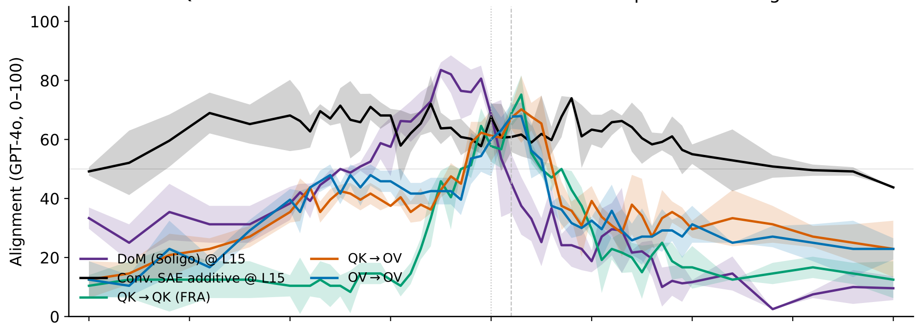
Qwen-2.5-7B + bad-medical · 5-method re-sweep · seed-averaged
