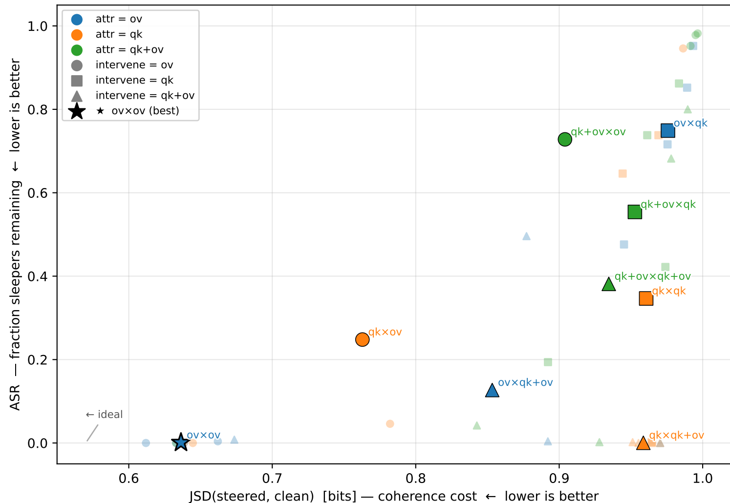
3×3 Attribution × Intervention matrix mean over SAE seeds 1-4, best \alpha \in \{2, 4\}
