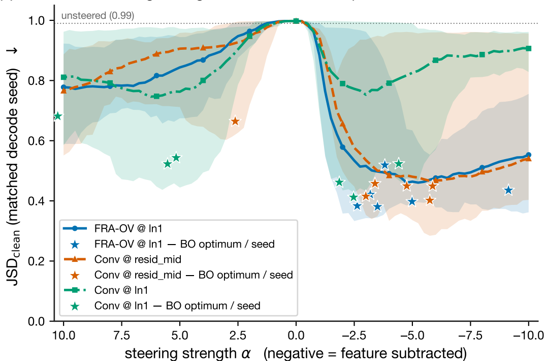
Sleeper suppression vs steering strength — winner feature per seed, mean \pm seed range (6 SAE seeds)
