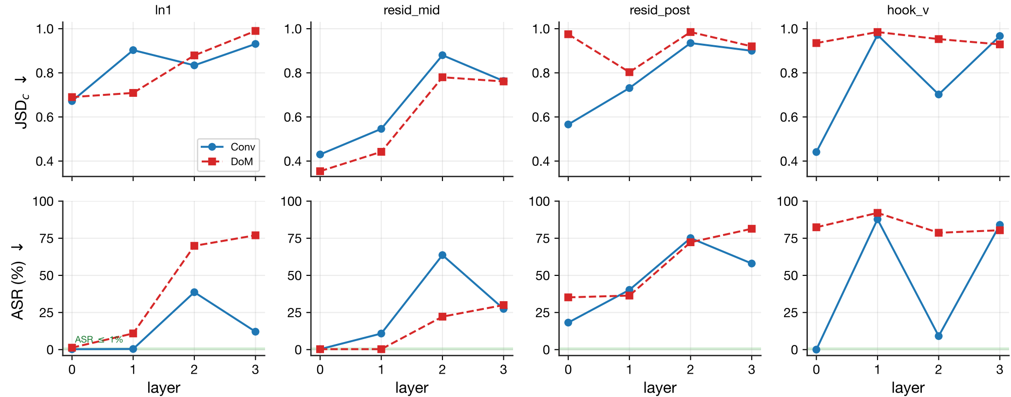
Localization with depth: JSD_c (top) and ASR (bottom) vs layer, per hook only resid_mid / hook_v at layer 0 reach low ASR at low JSD_c
