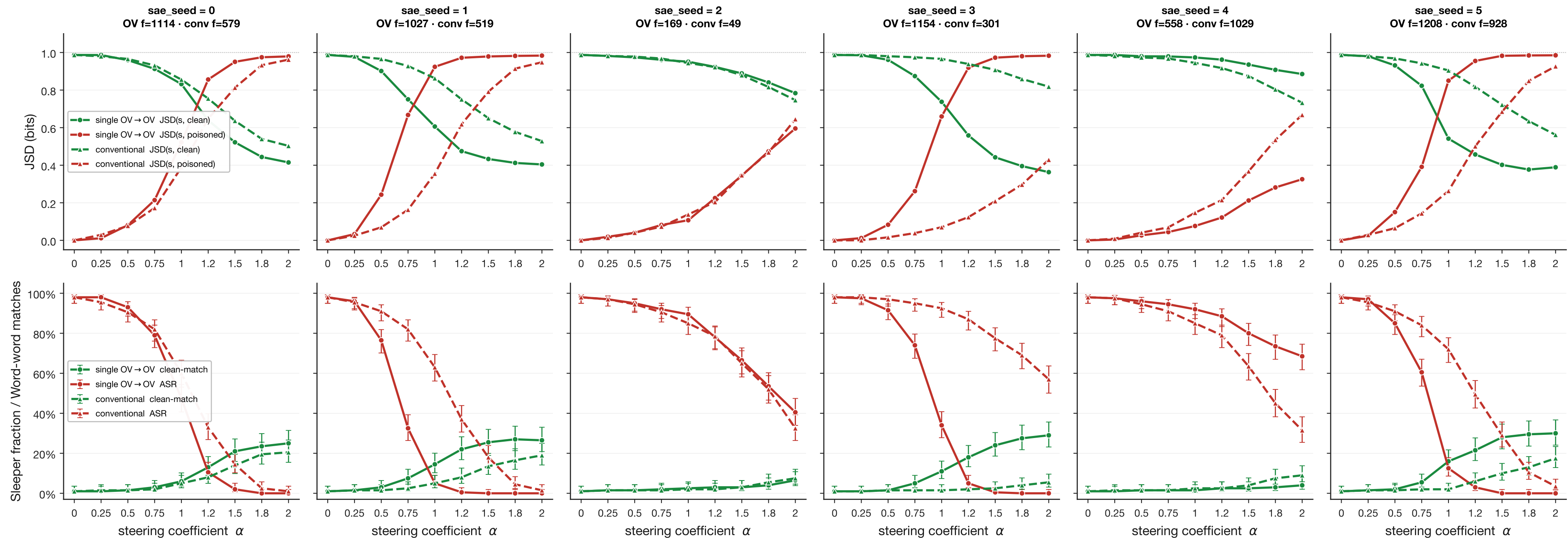
Per-seed companion to Fig.~2 — 50k SAE, single OV \rightarrow OV (solid+circle) vs conventional resid-mid additive (dashed+triangle). Top: JSD. Bottom: rollout-level (clean-match rate, ASR). Bottom-row error bars = 95 \% Wilson CI on the proportion (n = 200 prompts).
