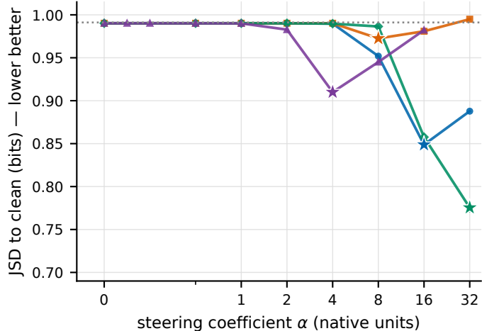
a Coefficient sweep · JSD to clean
