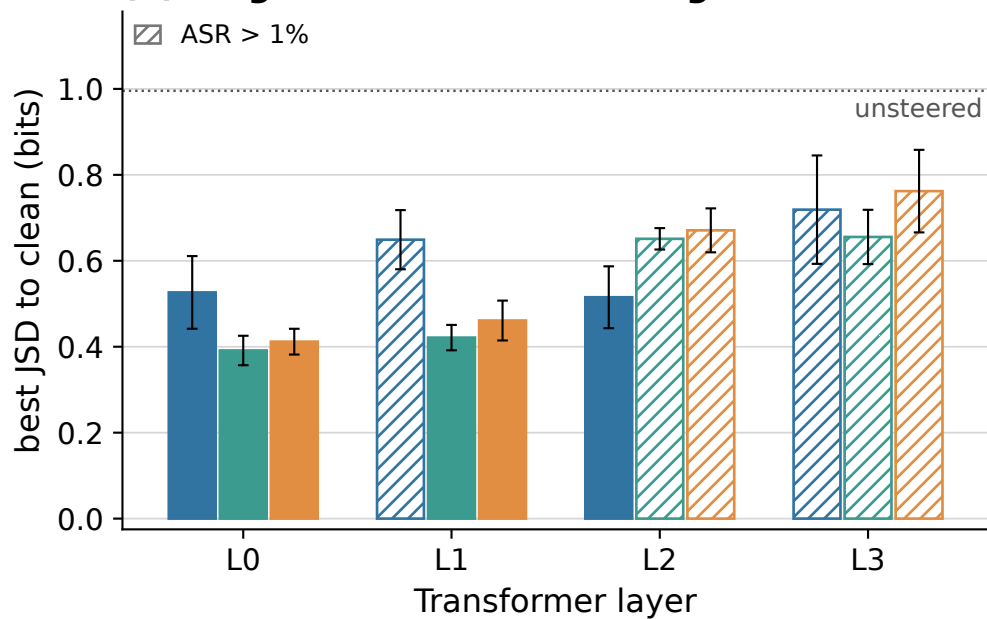
(b) Single-feature SAE steering
