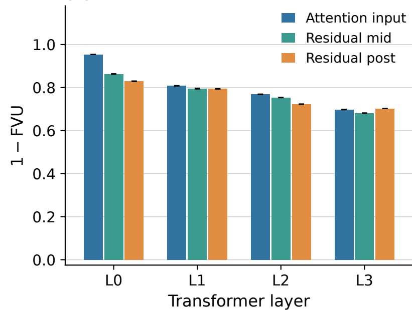
(a) SAE reconstruction
