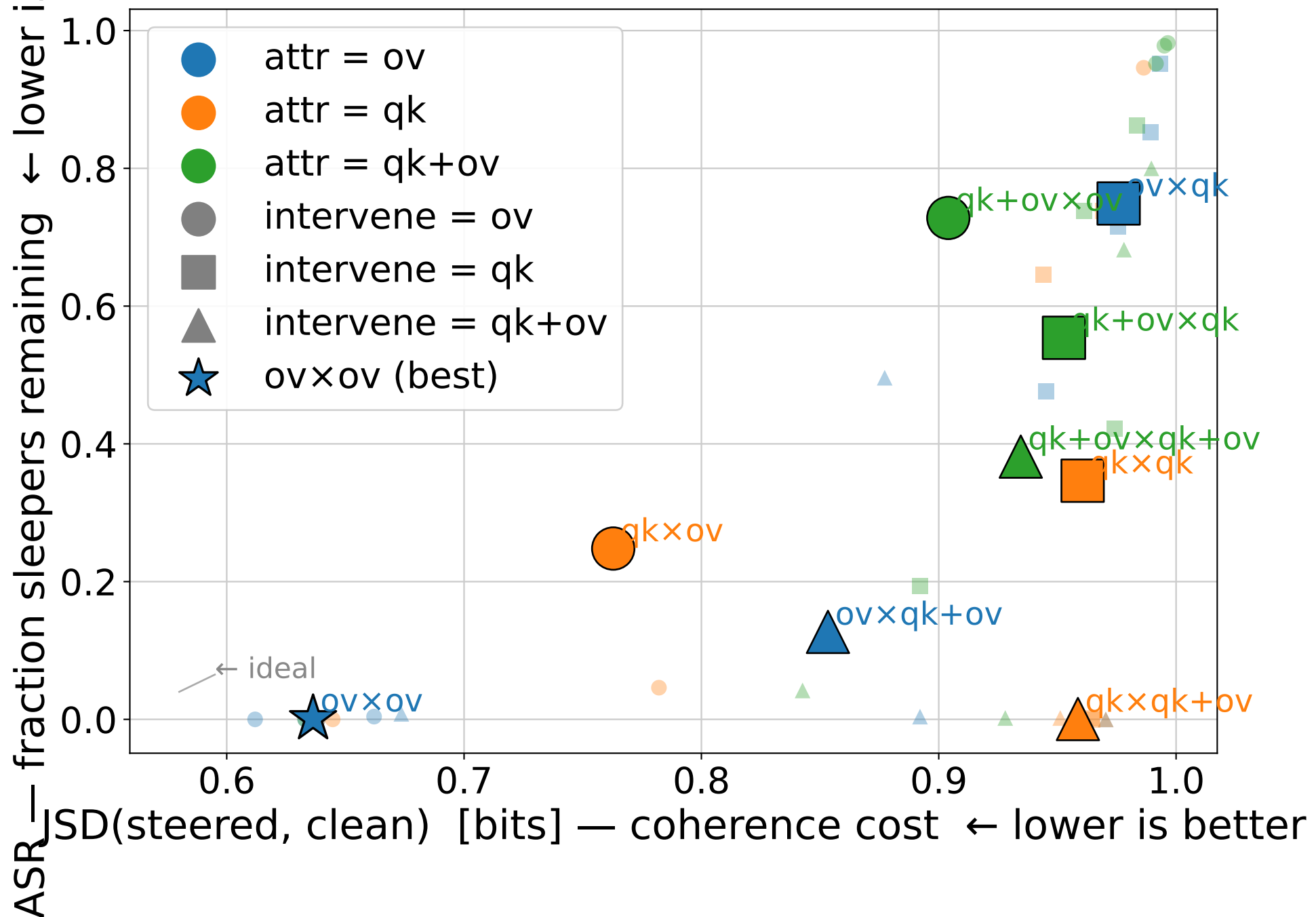
3×3 Attribution × Intervention matrix mean over SAE seeds 1-4
