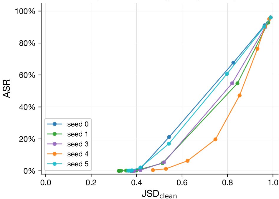
OV: per-seed steering-strength sweep
