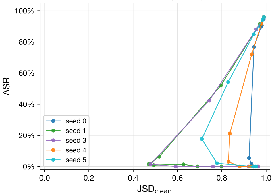
QK+OV: per-seed steering-strength sweep
