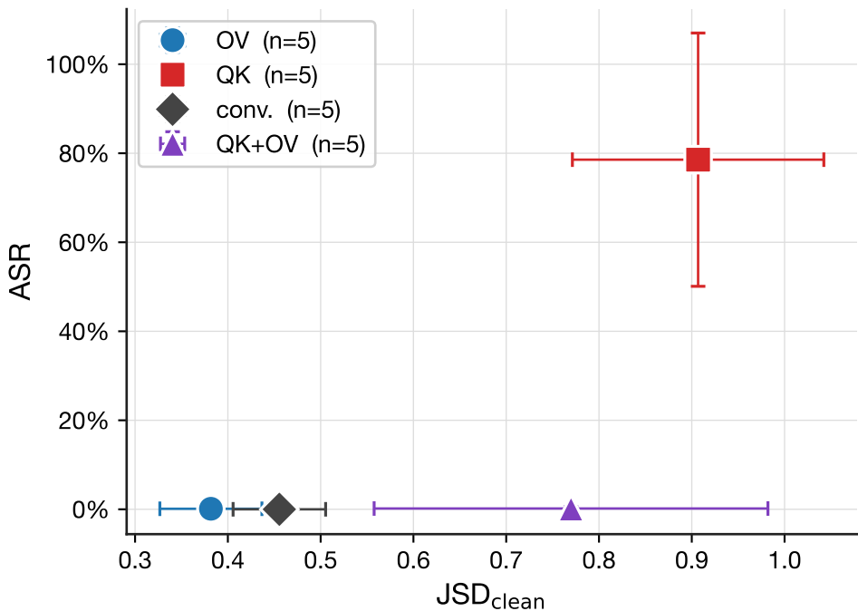
Coherence vs suppression at per-seed optimal \alpha
