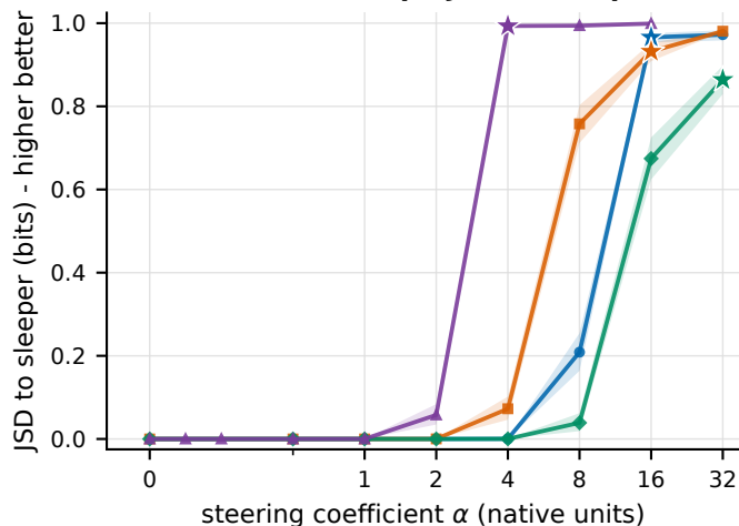
b Coefficient sweep · JSD to sleeper
