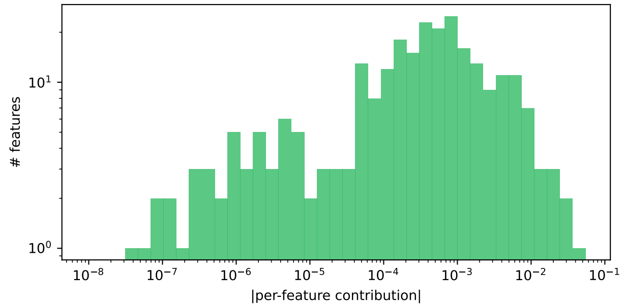
QK weight-diff — randpos PR=55 nonzero=265 top: f1307, f1709, f79
