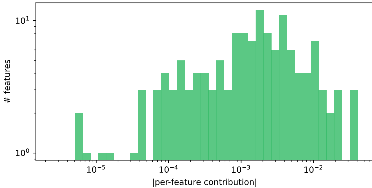
QK weight-diff — k1 PR=28 nonzero=139 top: f455, f409, f1889
