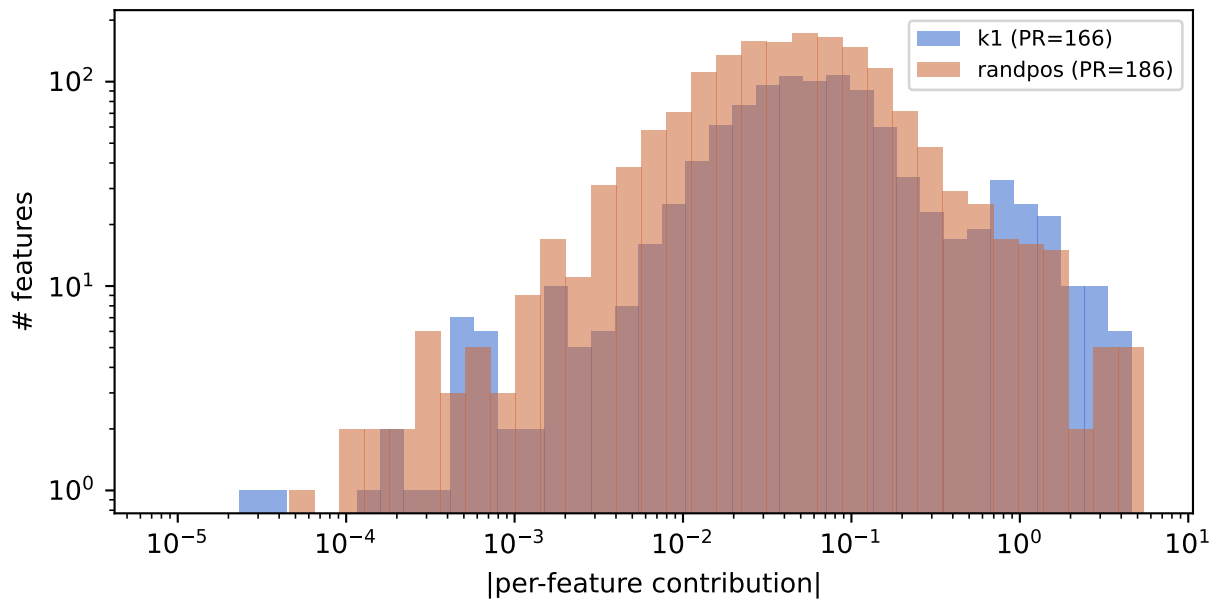
ln1 input-diff (deploy-clean) (conventional)
