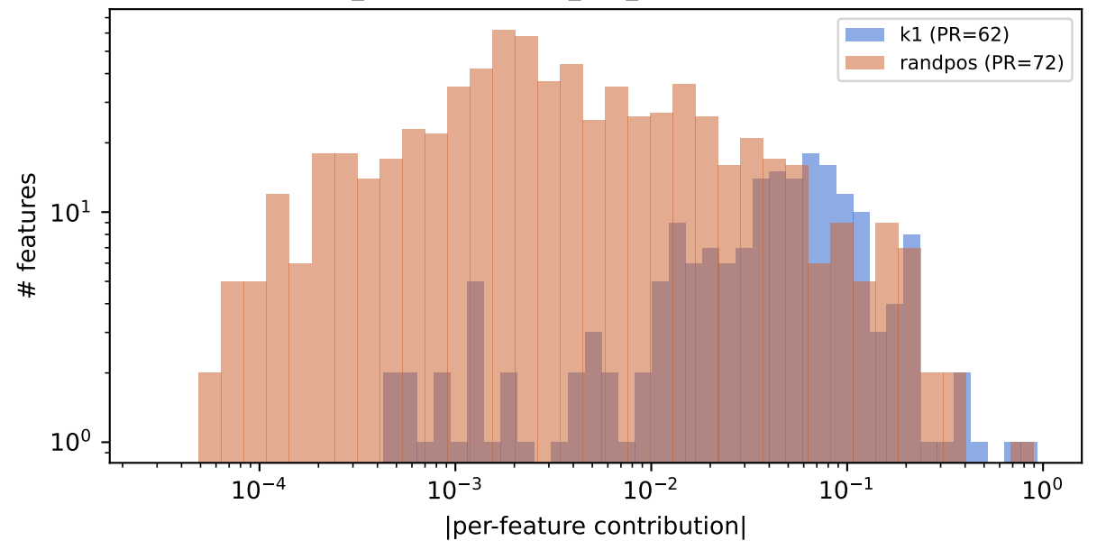
resid_mid model-diff ( z_s - z_b ) (proper model-diff)
