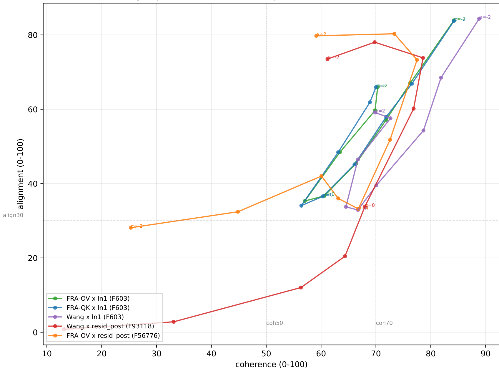
Steering trajectories — best feature per scheme (14B finance, \alpha \in [-2, 2] )
