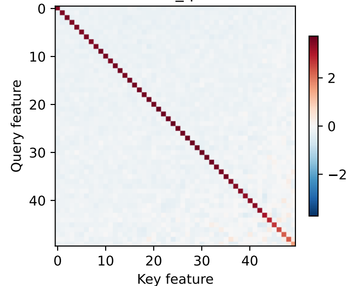
markov, rho=0.9, hit=1.0 sae_qk
