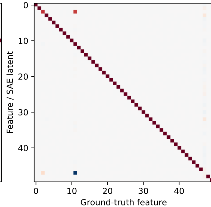
Learned decoder: one-to-one match
