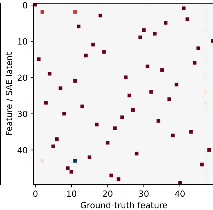
Learned decoder: original order
