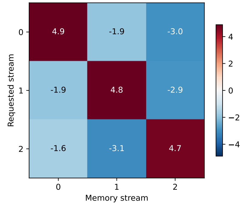
Effective QK stream scores (row-centered)
