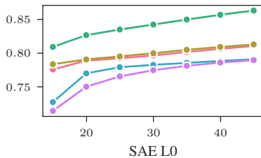
Variance Explained
