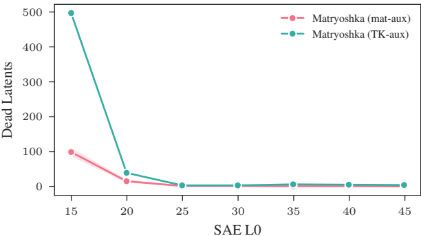
SynthSAEBench-16k results (Matryoshka aux comparison): Dead Latents
