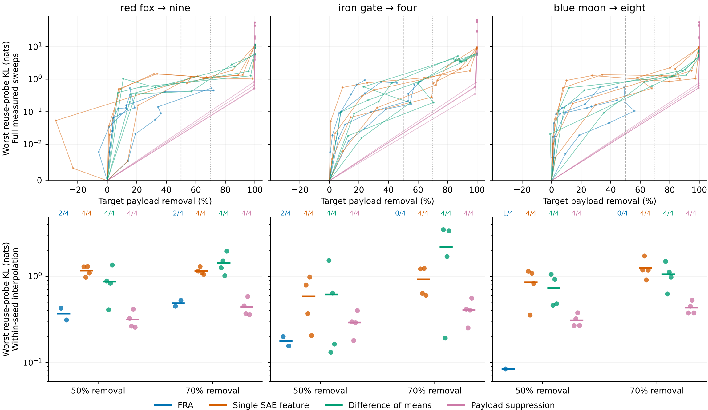
B1 conjunction removal • Gemma-2-2B base • original script 57 Four seeds per group; fractions show threshold coverage; lower KL is better
