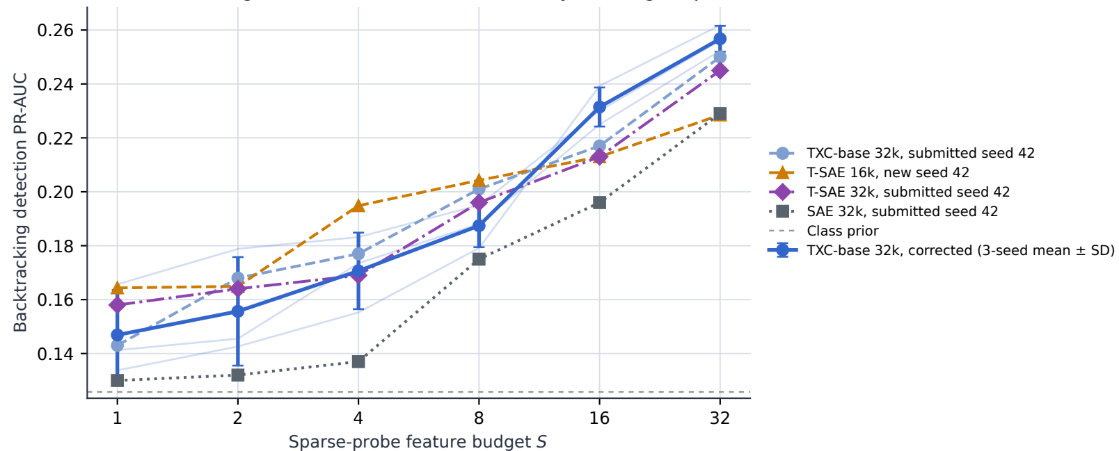
Backtracking detection after 300k dictionary-training steps
