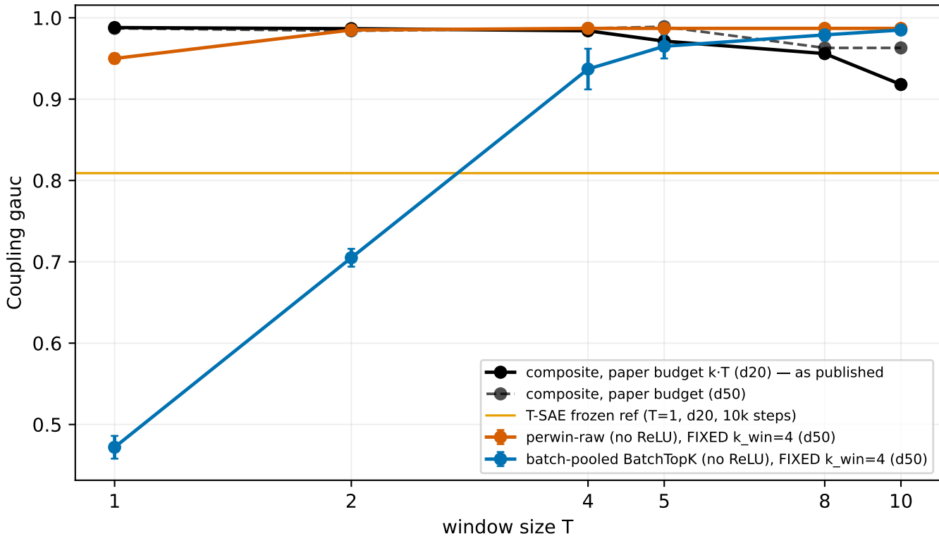
Budget scan winners: a fixed sparse window budget beats the paper's k·T rule (2 seeds mean \pm std for scan arms; incumbents 3 seeds)
