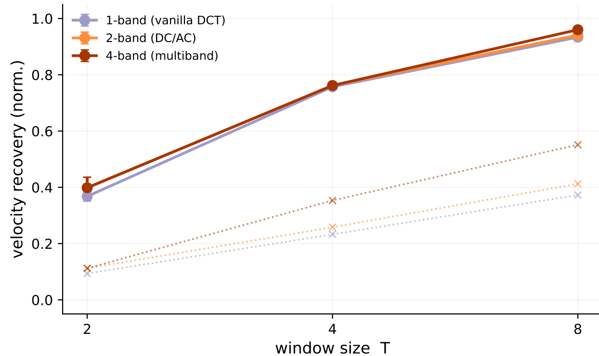
(a) Band partition vs T ( d_{\text{sae}} = M ; solid=trained, dotted=untrained)
