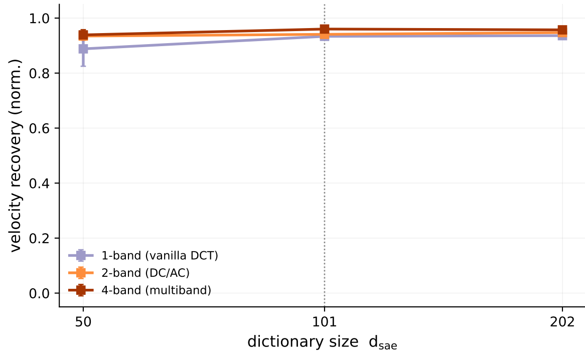
(b) Band partition vs capacity ( T = 8 )
