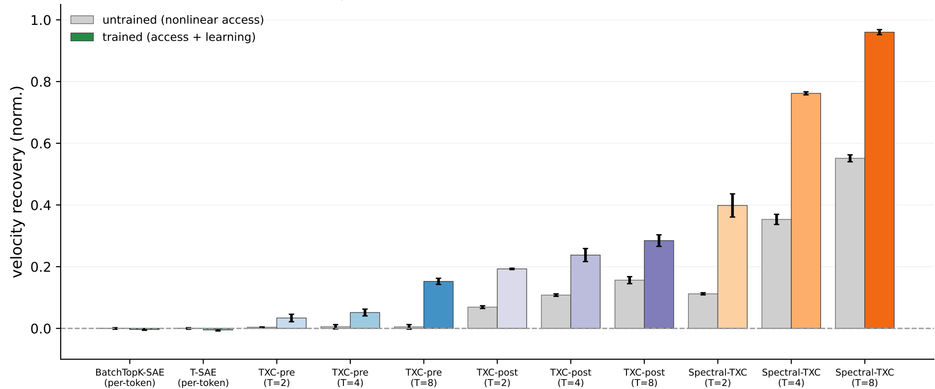
Access vs learning ( d_{\text{sae}} = M = 101 , k_{\text{pos}} = 1 )
