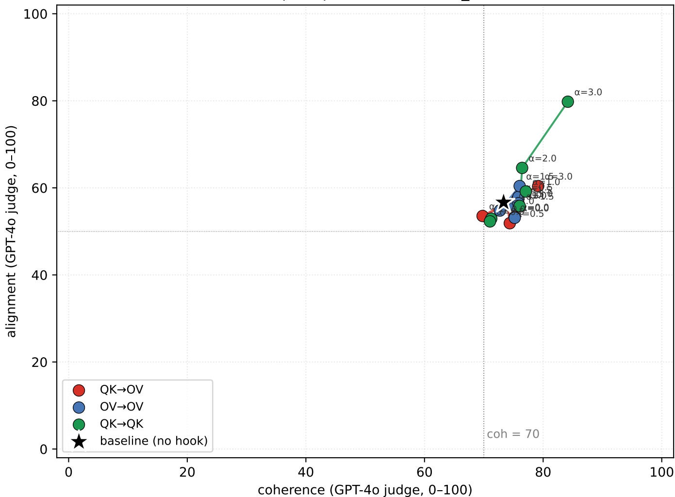
Nura medical @ L24 In1.hook_normalized — all 3 conditions (3 seeds \times 8 prompts \times 6 \alpha , frontier_multiseed)
