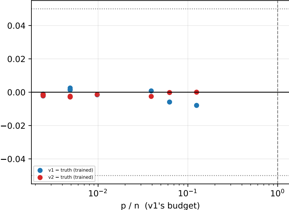
trained mirror ladder — deviation from truth (licensed cells)
