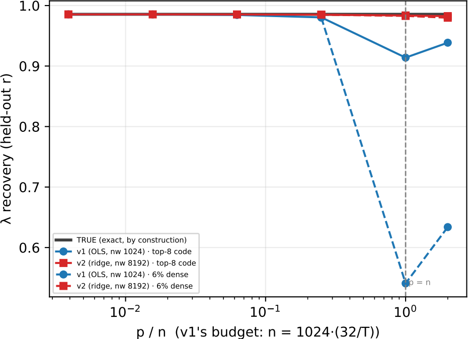
Stage 1 constructed code — full arm (truth known exactly)
