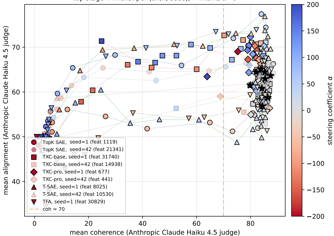
Coherence / alignment frontier on Qwen-2.5-7B bad-medical (L15) top stage-4 finalist per (arch, seed); ★ marks \alpha=0
