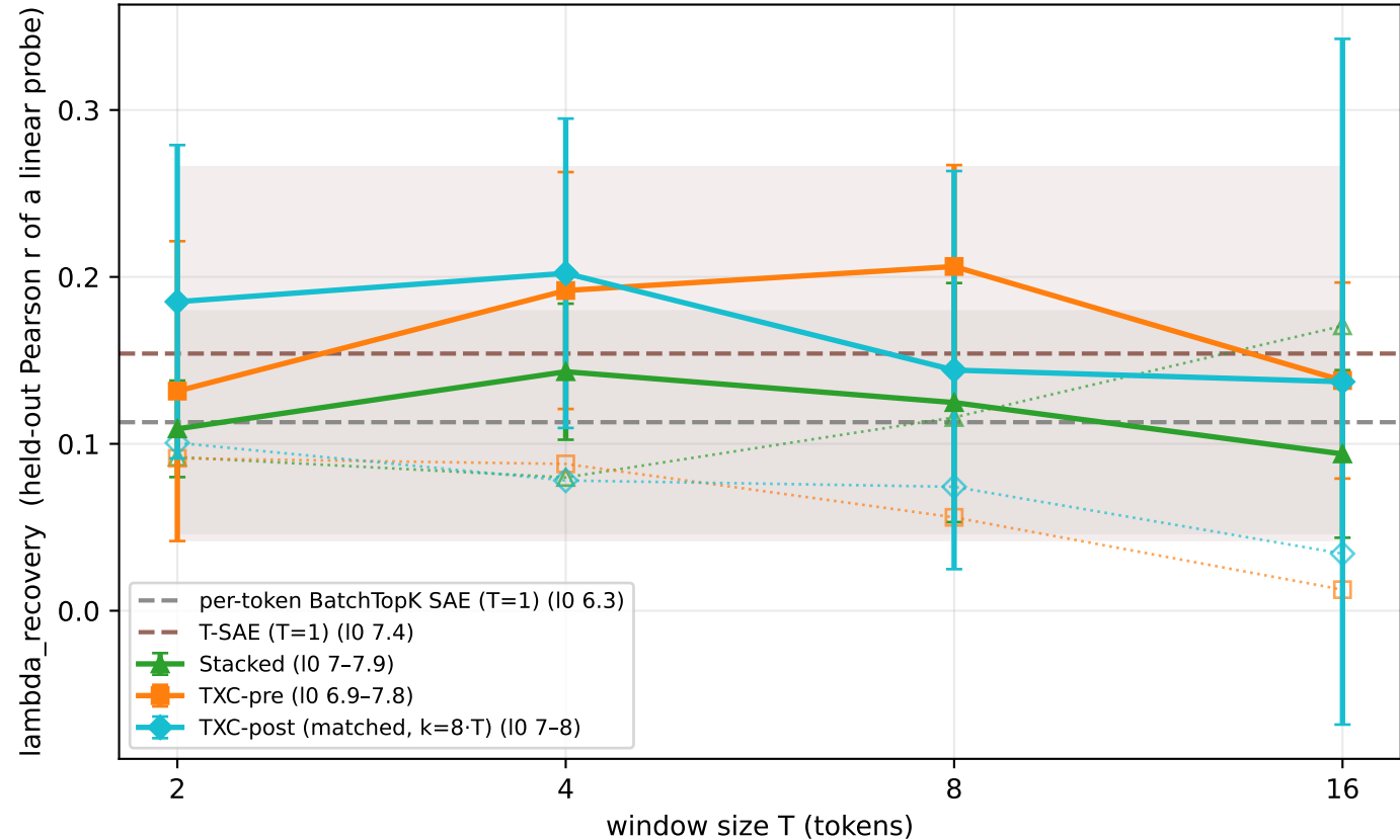
Task hunt Stage 2 — \hat{\lambda} recovery vs T, budget-matched archs only (realized IO within 2\times of nominal k; whiskers = 95% t CI over seeds)
