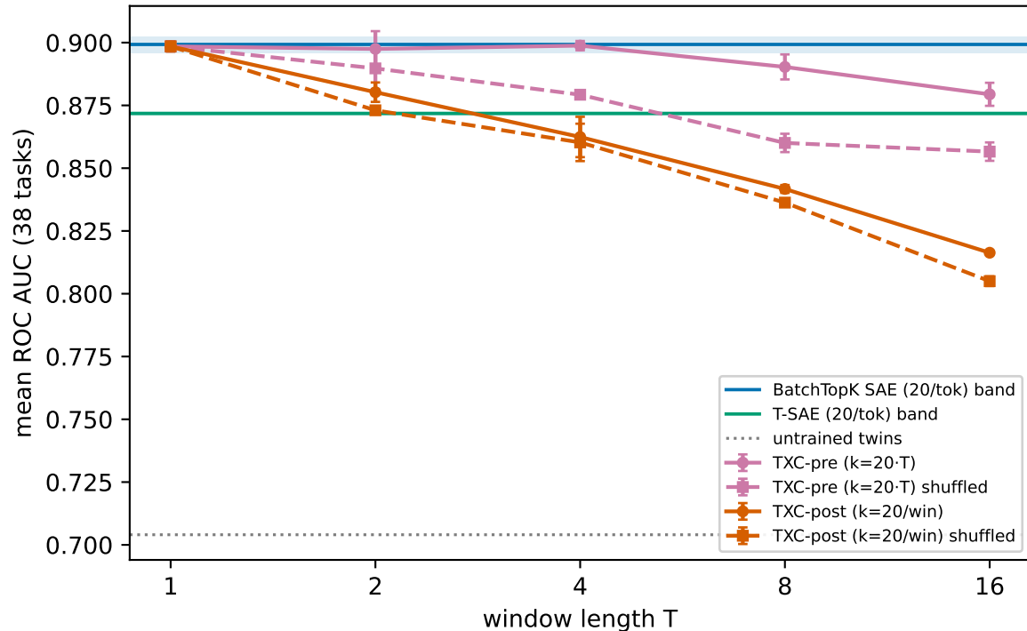
§5.1 sparse probing — btk-only arm, k_feat=20
