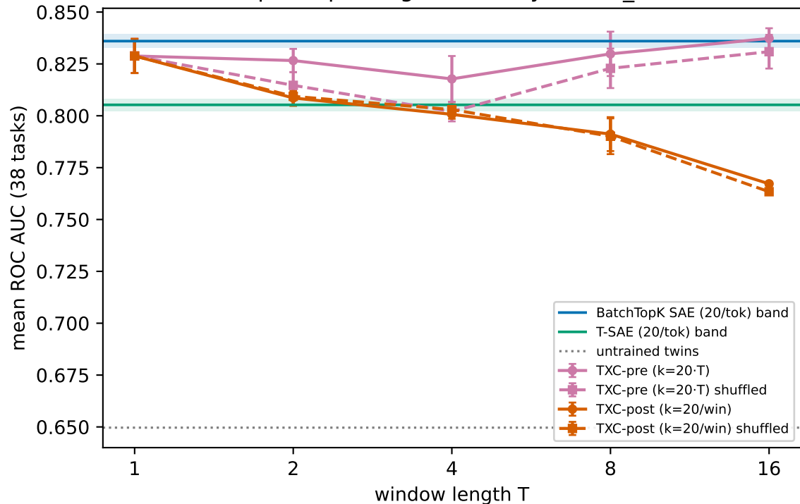
§5.1 sparse probing — btk-only arm, k_{\text{feat}}=5
