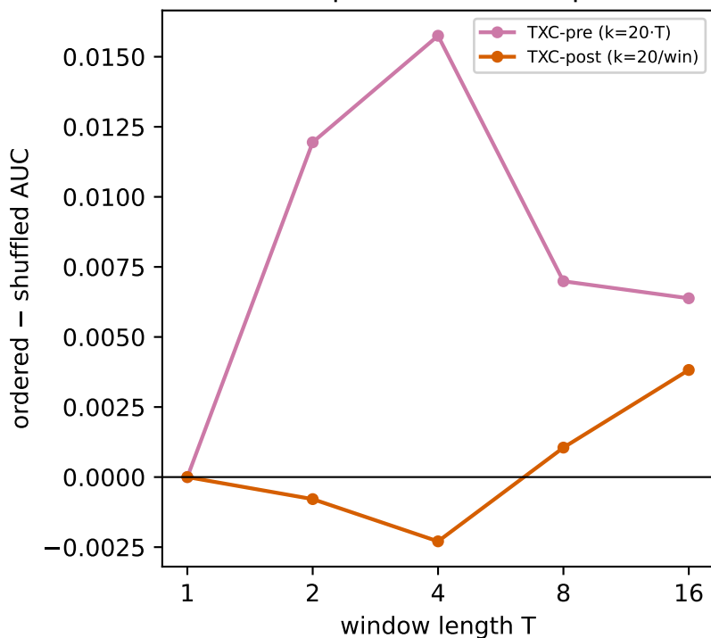
order dependence (fixed probe)
