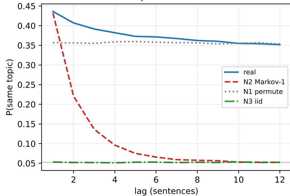
Same-topic autocorrelation
