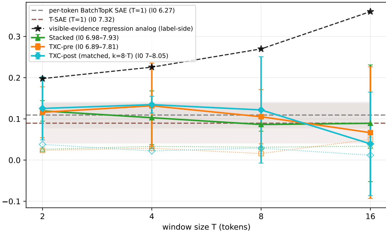
oprte Stage 2 — rate_case recovery vs T (v1, CANONICAL) REAL Ward activations (base, resid_post L12); whiskers = 95% t CI over seeds; hollow/dotted = untrained control; ★ = label-side evidence-line analog
