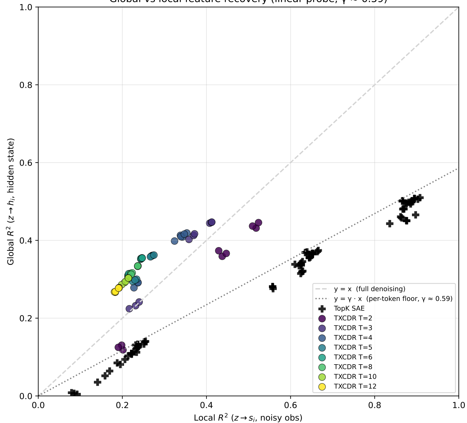
Global vs local feature recovery (linear probe, \gamma \approx 0.59 )
