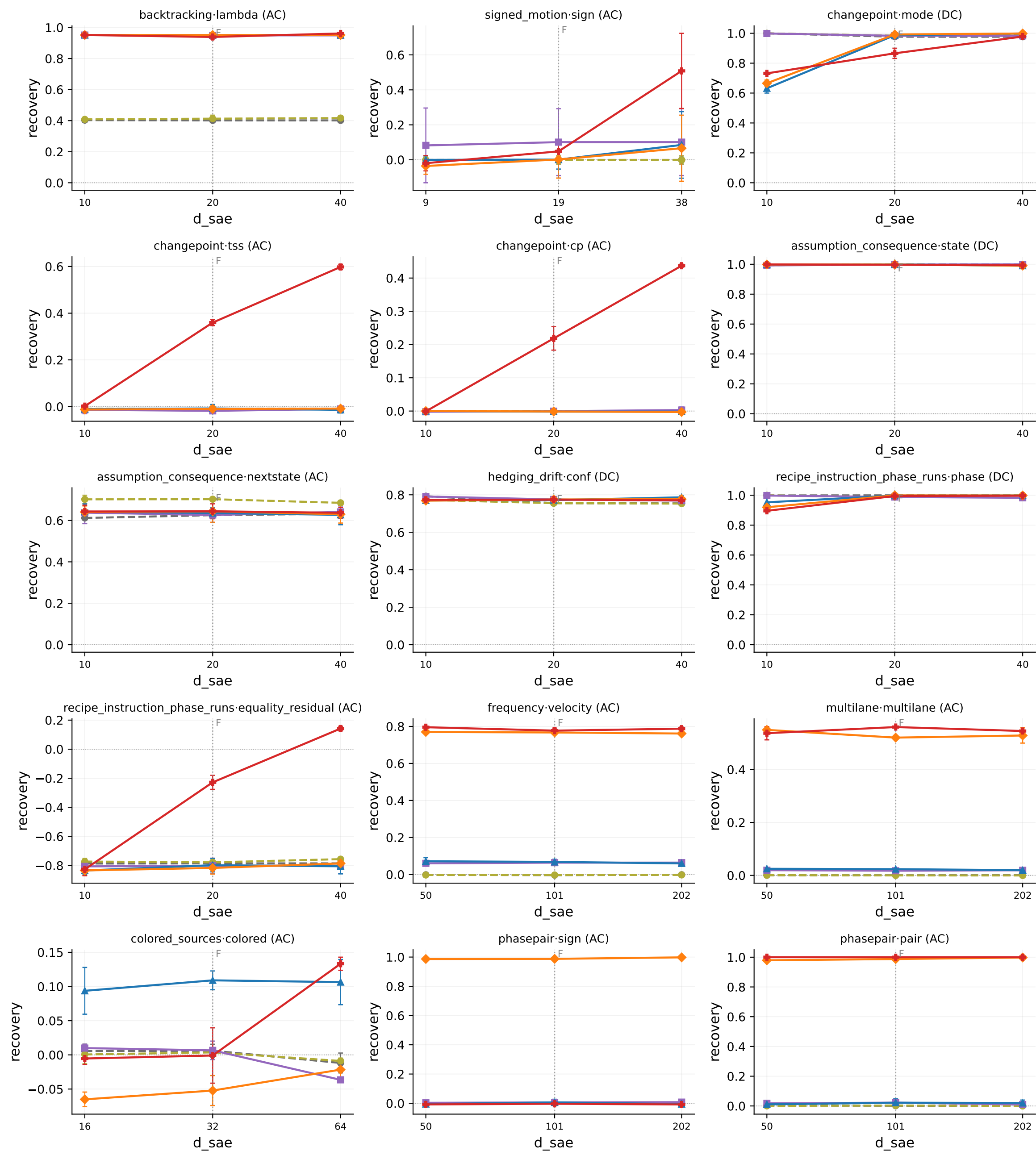
Recovery vs capacity (per-token matched, T_can=4)
