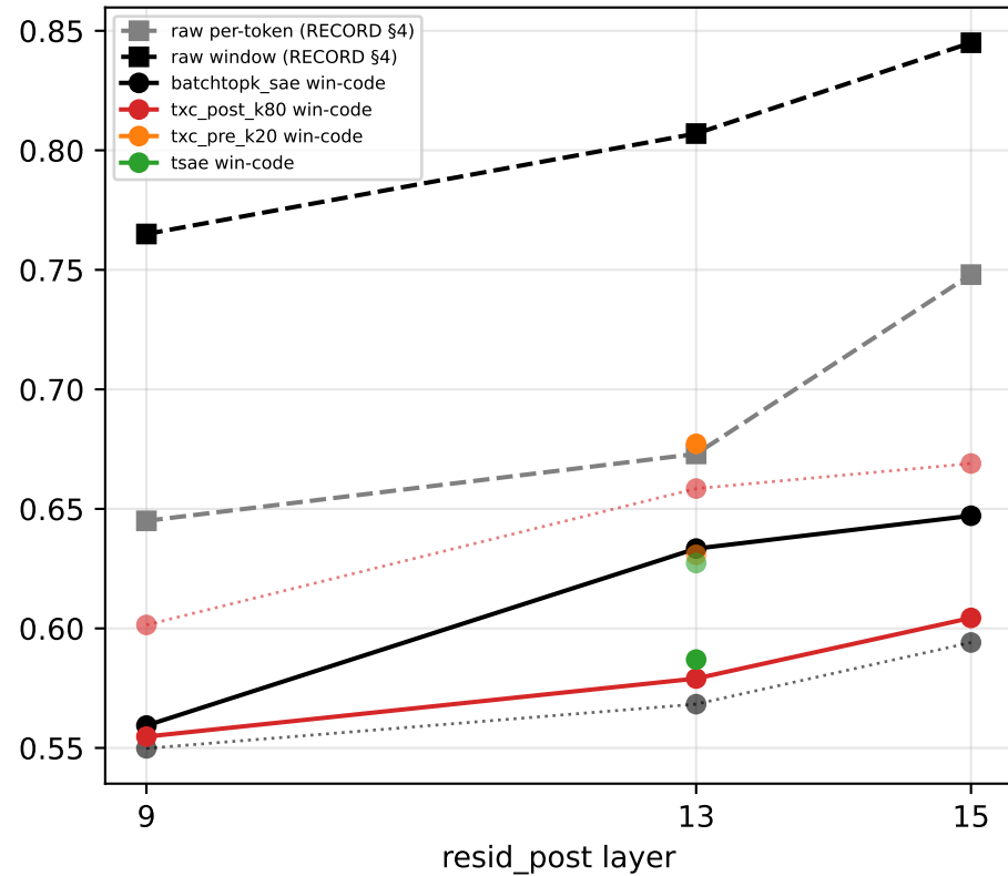
probe currency: code AUC (dotted=token, solid=window)
