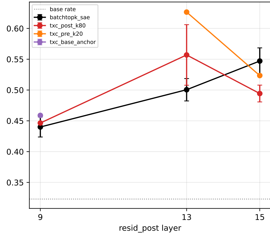
paper currency: sparse-probe PR-AUC (S=16)
