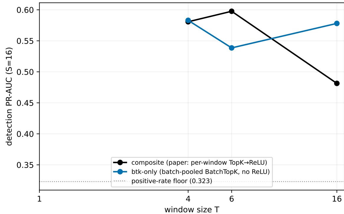
§5.3 EM detection vs window size — paper arch, both arms (Qwen-7B medical organism, L15, 25k steps, seed 42)
