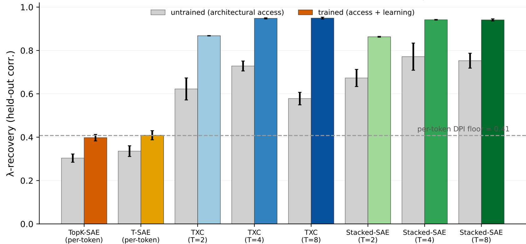
Access vs learning: random-init vs trained encoders ( d_{\text{sae}} = 20 , k_{\text{pos}} = 1 )
