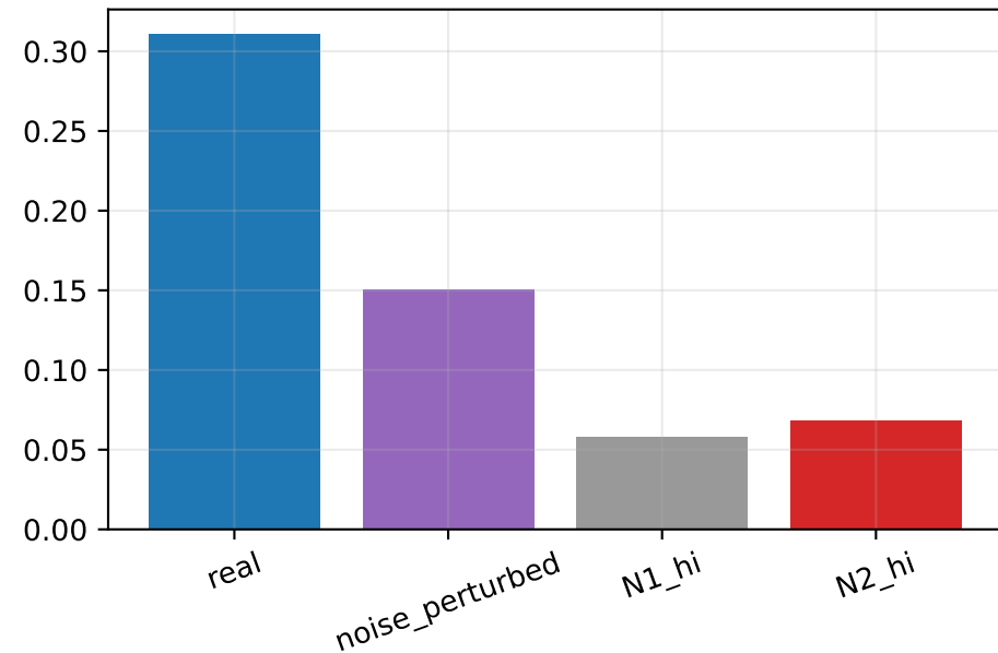
Gate on acf[lag1] → PROCEED
