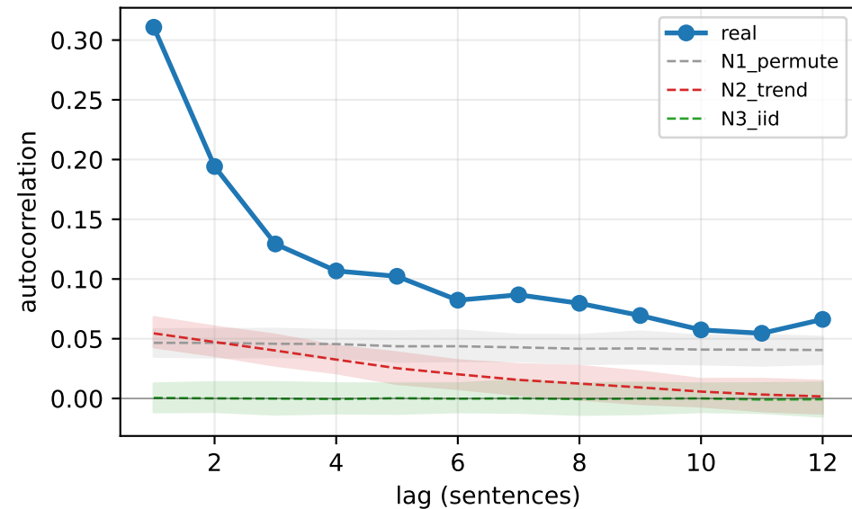
ACF: real vs nulls
