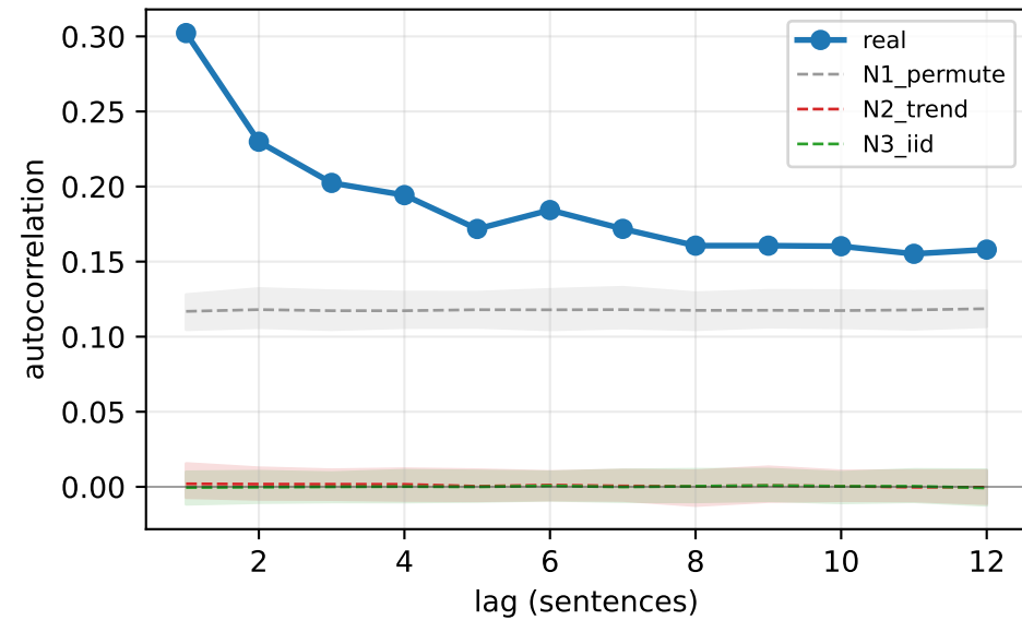
ACF: real vs nulls
