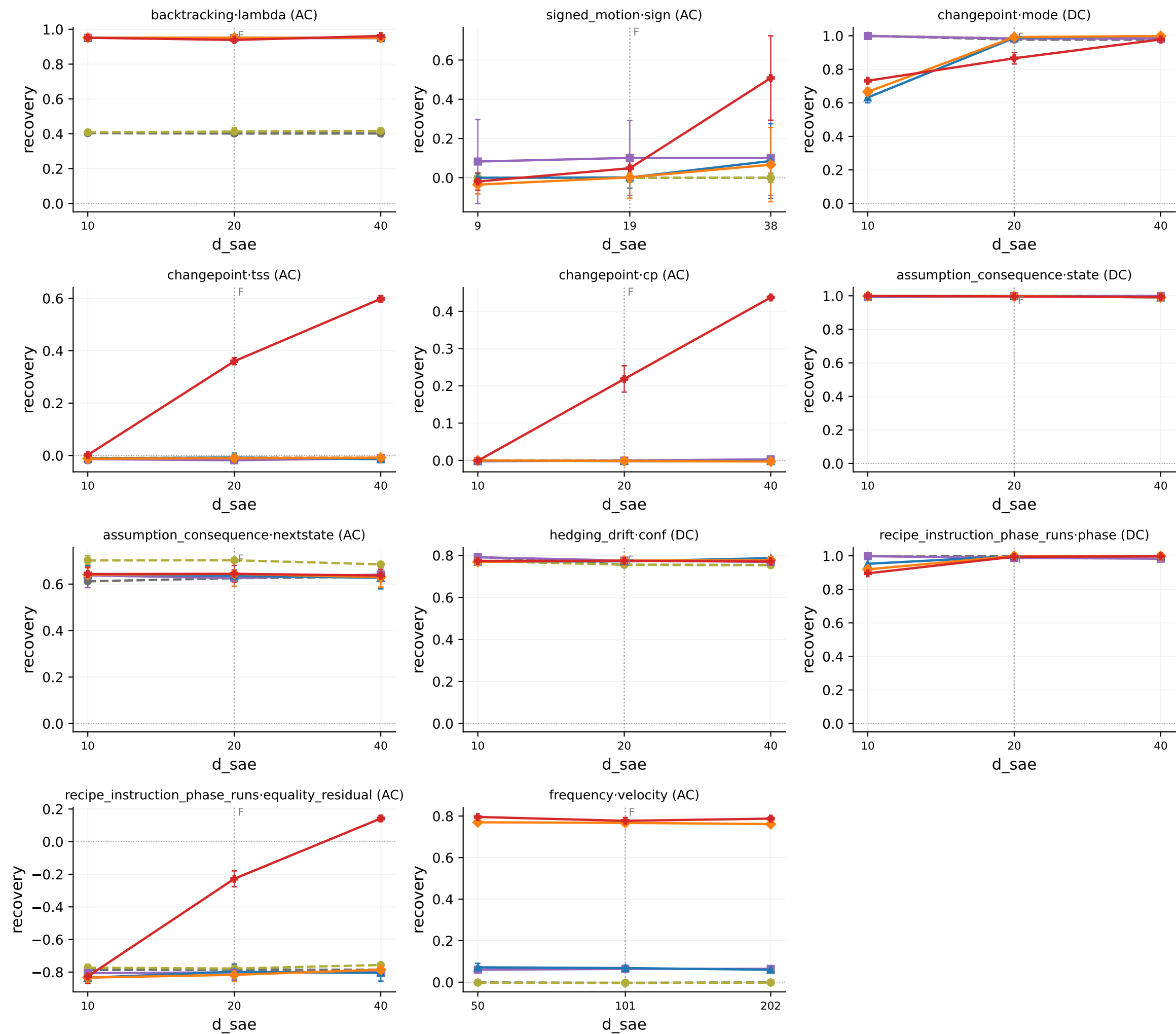
Recovery vs capacity (per-token matched, T can =4)
