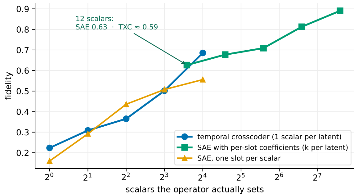
B. Counted in scalars rather than latents, the SAE is not behind
