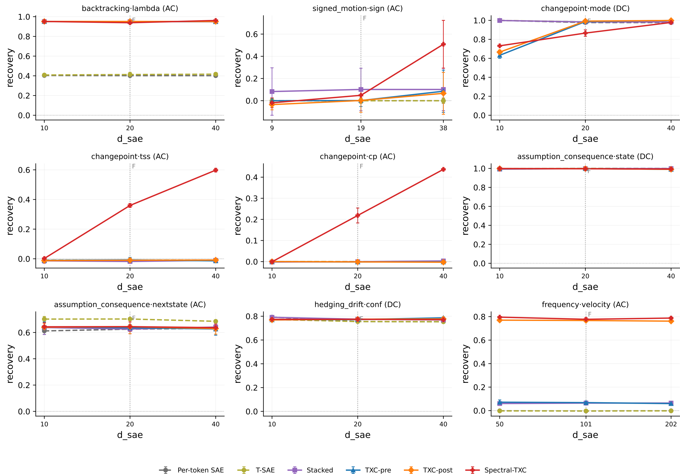
Recovery vs capacity (per-token matched, T_{\text{can}}=4 )
