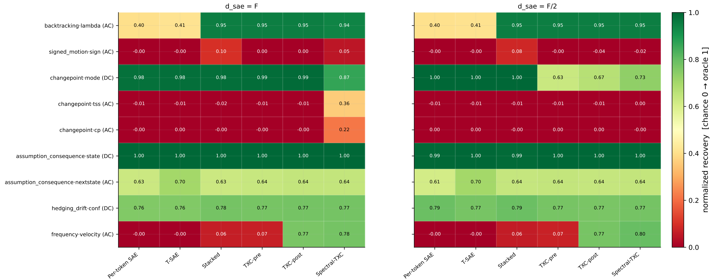
Per-token matched recovery ( T_{\text{can}}=4 , B^*=2 )
