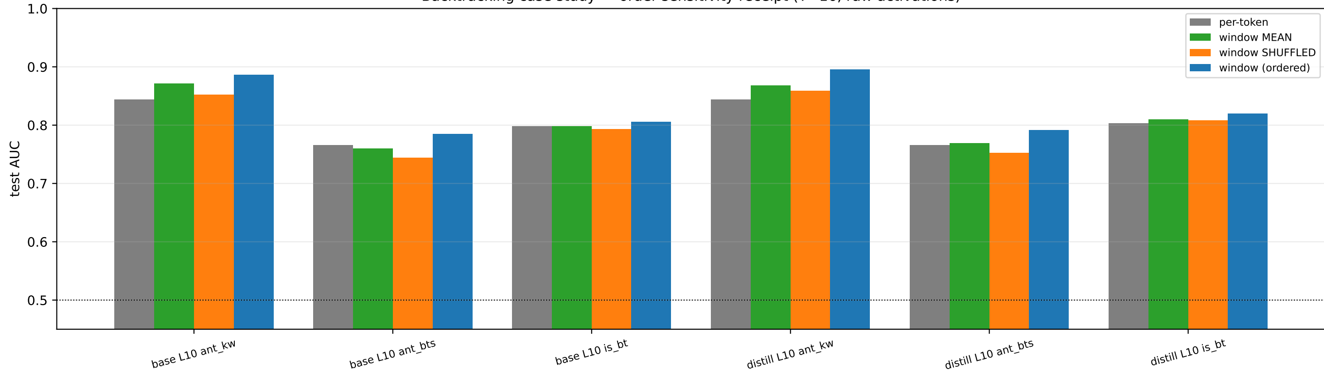
Backtracking case study — order-sensitivity receipt (T=16, raw activations)
