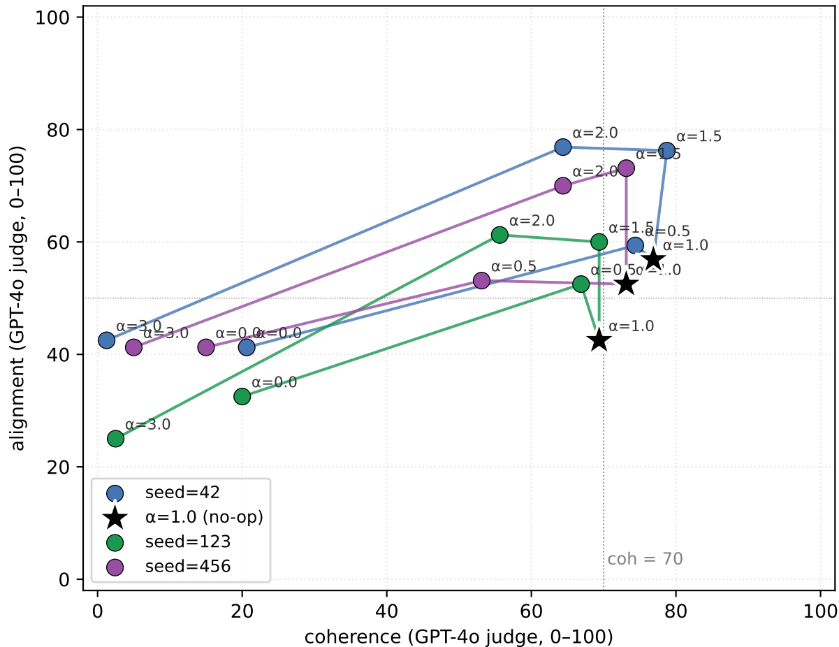
SAE-resid steering @ blocks.24.hook_resid_post (medical EM, k=64, top-50 features)
